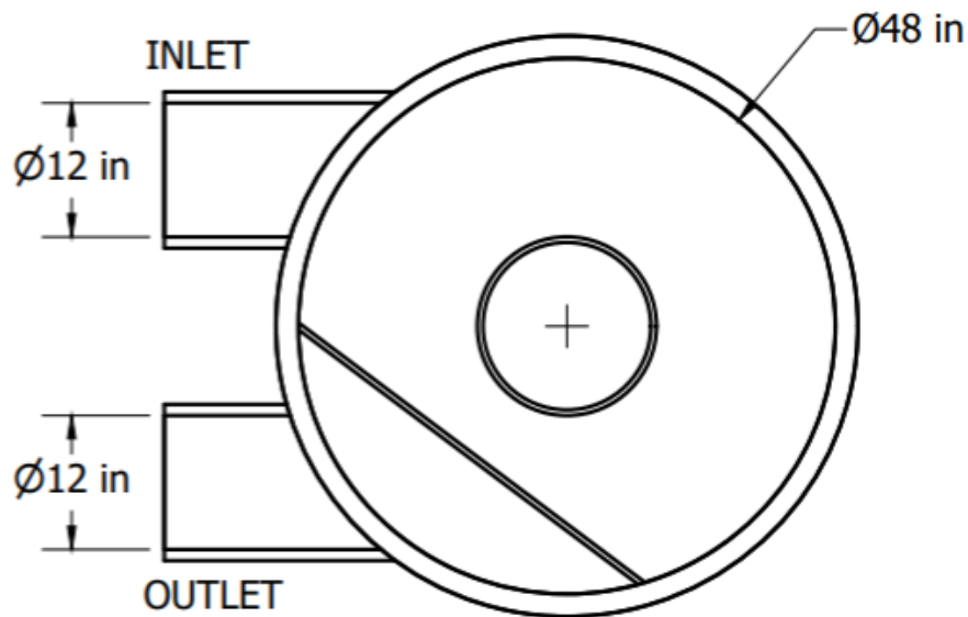
Figure 2 Plan View of the Arcadia in Horseshoe Configuration
