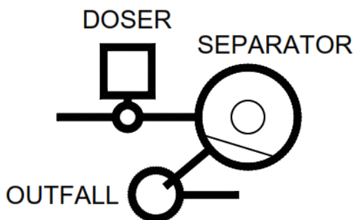
Figure 4 Plan View Schematic Detail of the Arcadia Angled Inlet Test Configuration
