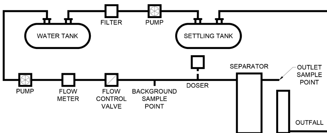
Figure 3 Schematic of the Arcadia Test Configuration
