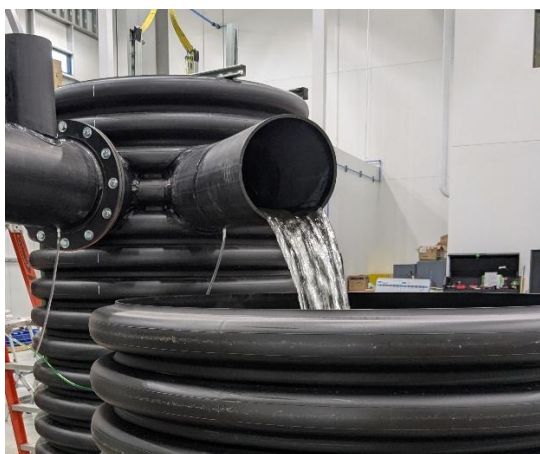
Figure 6 Photo of the Arcadia Angled Inlet Test Configuration
