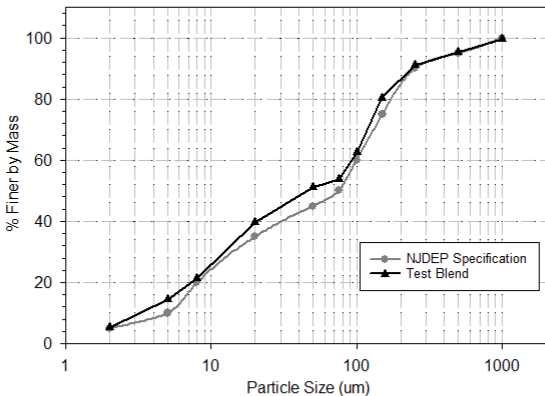
Figure 8 Average PSD of Removal Efficiency Sediment vs NJDEP Protocol Specification
