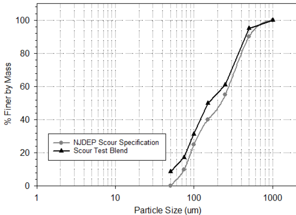
Figure 9 Average PSD of Scour Sediment vs NJDEP Protocol Specification
