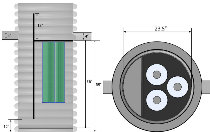
Figure 2: Profile View and Plan View of ALUX-3M Test Unit
