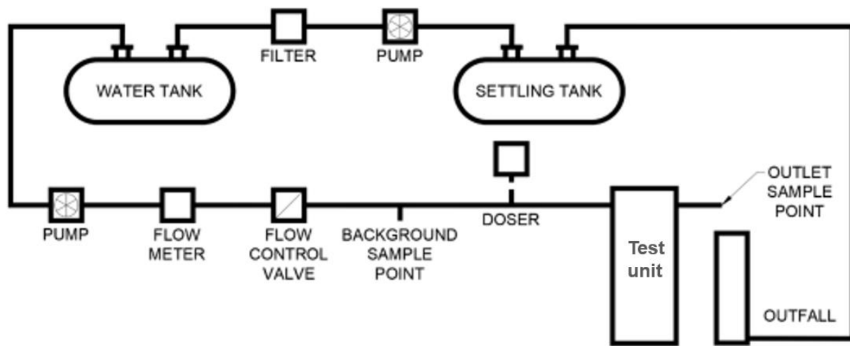
Figure 3: Schematic of the ALUX-3M Test Configuration
